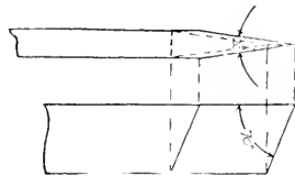
FIG. 127. SMALL SKEW— ANGLE FOR SOFT WOOD.
